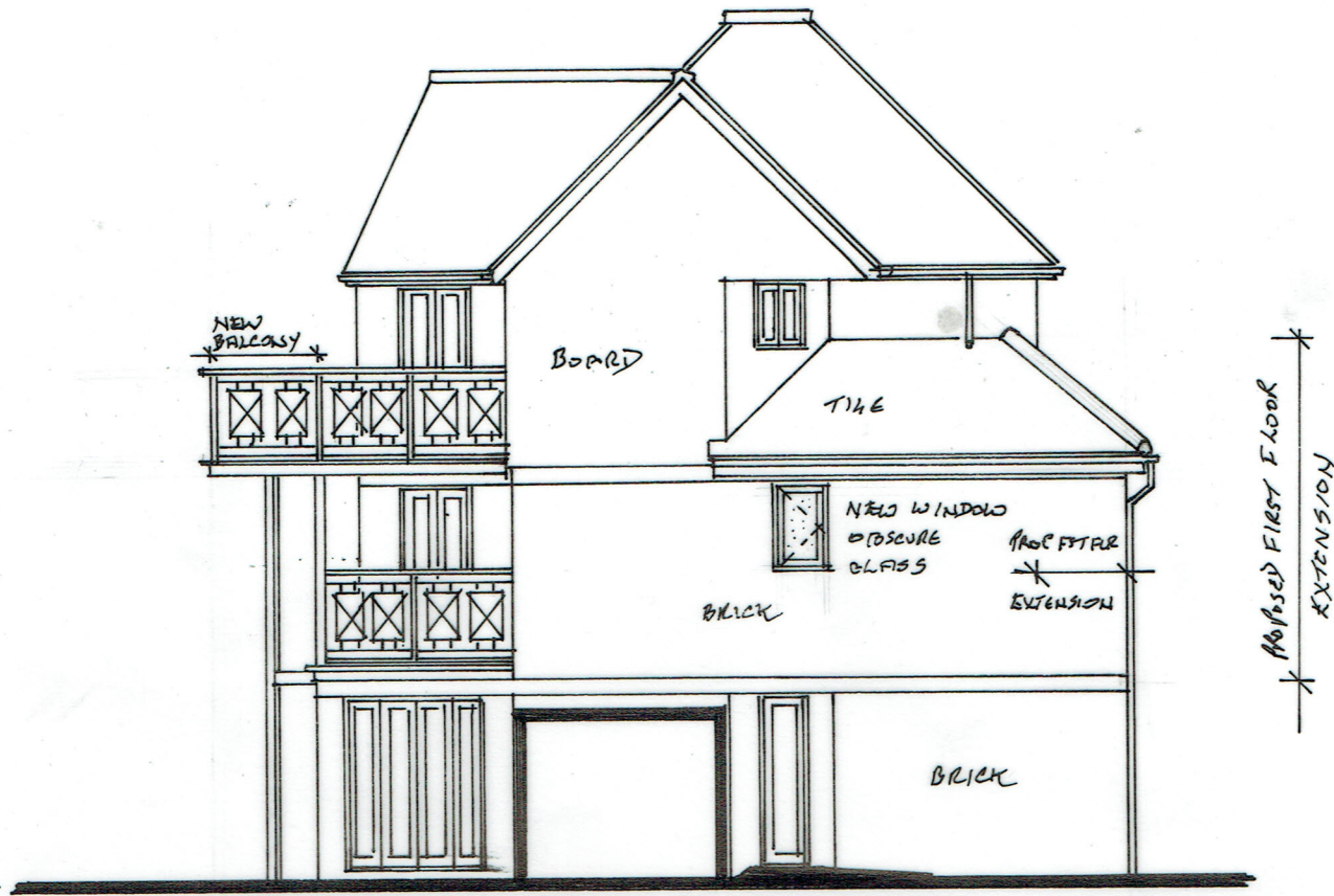
PROPOSED NORTH WEST ELEVATION (SIDE)
